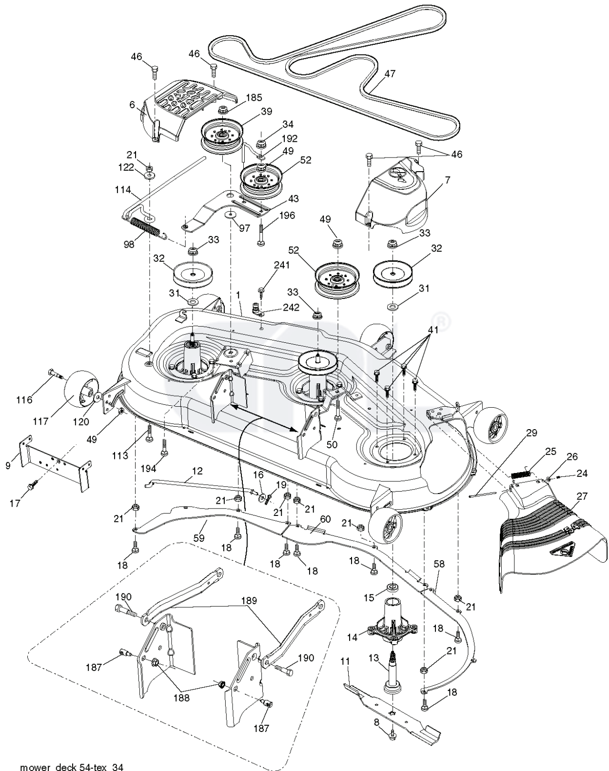
mower_deck 54-tex_34
