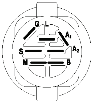
IGNITION SWITCH
